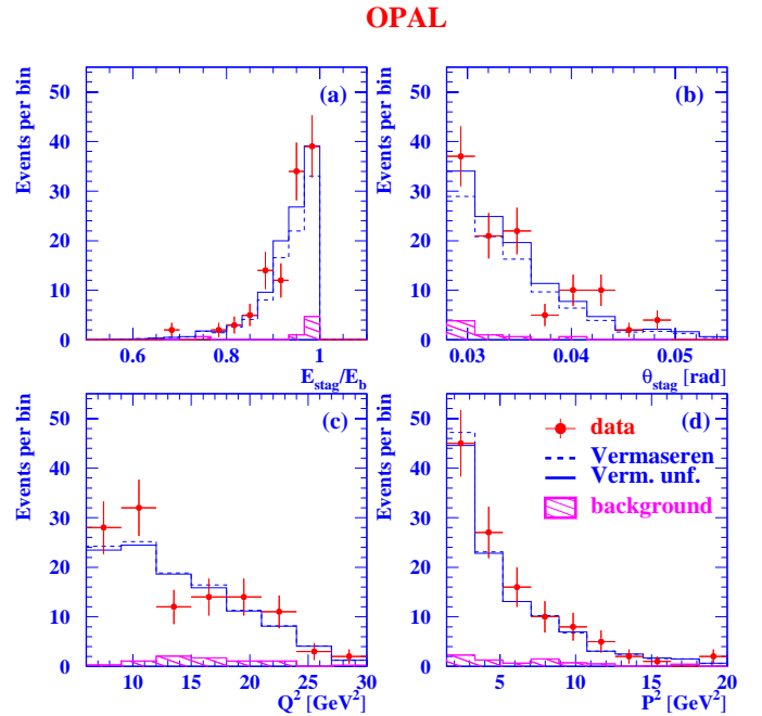
Fig. 4. Comparison of the data with the Monte Carlo predictions for the DB samples. Figures a, b and c, d are for the DB1 and DB2 samples, respectively. Shown are a the energy of the second detected electron normalised to the energy of the beam electrons, E_{\text{stag}}/E_b , b the polar angle of the second detected electron, \theta_{\text{stag}} , c the measured Q^2 , and d the measured P^2 . The points represent the data with the statistical error only. The dashed lines denote the distributions of the Vermaseren Monte Carlo with the background added to it before the unfolding is performed, the full lines are the same distributions after reweighting based on the unfolding procedure, and the hatched histograms represent the background contribution
