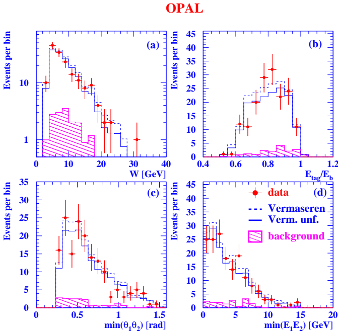
Fig. 3. Comparison of the data with the Monte Carlo predictions for the EE sample. Shown are a the measured invariant mass, W , b the energy of the detected electron normalised to the energy of the beam electrons, E_{\text{tag}}/E_b , c the polar angle of the muon which is scattered closer to the beam direction, \min(\theta_1, \theta_2) , and d the energy of the muon with lower energy, \min(E_1, E_2) . The points represent the data with the statistical error only. The dashed lines denote the distributions of the Vermaseren Monte Carlo with the background added to it before the unfolding is performed, the full lines are the same distributions after reweighting based on the unfolding procedure, and the hatched histograms represent the background contribution
