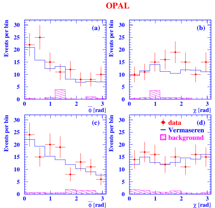
Fig. 5. Comparison of the data with the Monte Carlo predictions for the DB samples. Figures a,b and c,d are for the DB1 and DB2 samples, respectively. Shown are ( a,c ) the angle \bar{\phi} between the two scattering planes of the electrons in the photon-photon centre-of-mass system, and ( b,d ) the measured azimuthal angle, \chi , defined with respect to the plane containing the electron which radiated the photon of higher virtuality. The points represent the data with the statistical error only. The full lines denote the distributions of the Vermaseren Monte Carlo with the background added to it, and the hatched histograms represent the background contribution
