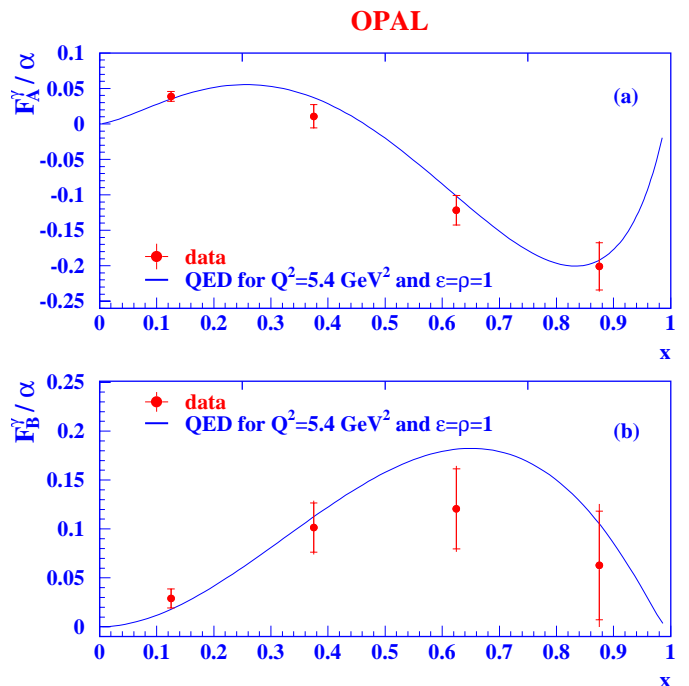
Fig. 15. The measured structure functions F_A^\gamma and F_B^\gamma for the combined SW and FD sample. The points represent the data with their statistical (inner error bars) and total errors (outer error bars). The solid lines are the QED predictions for Q^2 = 5.4 \text{ GeV}^2 and \epsilon = \rho = 1 . \chi^2/\text{dof} = 3.5/4 for F_A^\gamma and \chi^2/\text{dof} = 3.8/4 for F_B^\gamma
