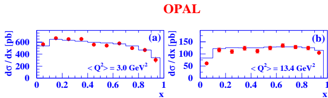
Fig. 8. Differential cross-sections d\sigma/dx unfolded from the data for the two combined samples of singly-tagged events. The samples shown are a SW and b FD. The symbols are as defined in Fig. 7
