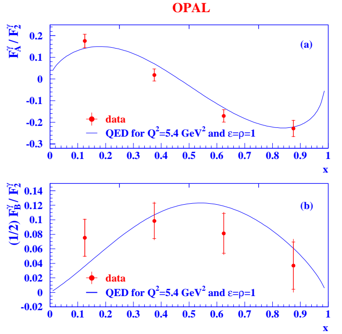
Fig. 14. The measured structure function ratios F_A^\gamma/F_2^\gamma and \frac{1}{2}F_B^\gamma/F_2^\gamma for the combined SW and FD sample. The points represent the data with their statistical (inner error bars) and total errors (outer error bars). The solid lines are the QED predictions for Q^2 = 5.4 \text{ GeV}^2 and \epsilon = \rho = 1 . \chi^2/\text{dof} = 5.9/4 for F_A^\gamma/F_2^\gamma and \chi^2/\text{dof} = 4.4/4 for \frac{1}{2}F_B^\gamma/F_2^\gamma
