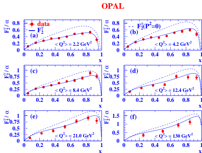
Fig. 9. Structure functions F_2^\gamma normalised by the fine structure constant \alpha for the various independent samples of singly-tagged events. The ordering of sub-figures is the same as in Fig. 7. The points represent the data with their statistical (inner error bars) and total errors (outer error bars). The full line is the structure function F_2^\gamma normalised by the fine structure constant \alpha for the \langle Q^2 \rangle and \langle P^2 \rangle values listed in Table 1, and the dashed line shows the structure function F_2^\gamma normalised by the fine structure constant \alpha for the same \langle Q^2 \rangle but for P^2 = 0 . The tic marks at the top of the figures indicate the bin boundaries
