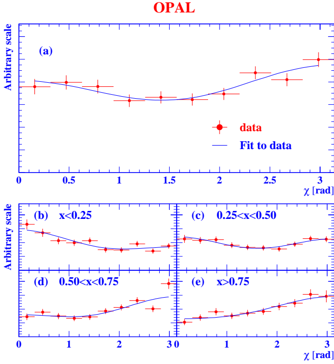
Fig. 13. Corrected azimuthal angle distributions for the combined SW and FD sample for different ranges of x . The points represent the corrected data with the statistical error only, and the full line is a fit to the data based on (14)
