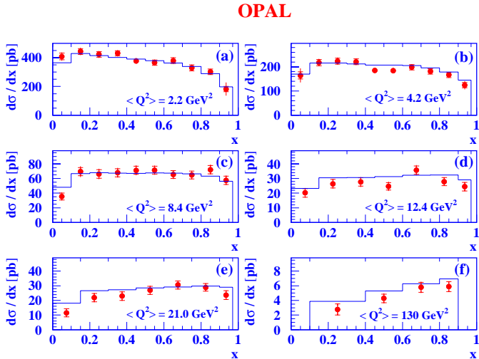
Fig. 7. Differential cross-sections d\sigma/dx unfolded from the data for the various independent samples of singly-tagged events. The samples shown are a SW1, b SW2, c FD1, d FD2, e FD3 and f EE. The points represent the data with their statistical (inner error bars) and total errors (outer error bars). The full line is the differential cross-sections as predicted by the Vermaseren Monte Carlo. The tic marks at the top of the figures indicate the bin boundaries
