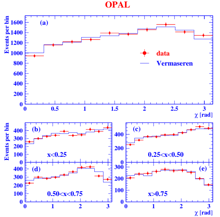
Fig. 12. Measured azimuthal angle distributions for the combined SW and FD sample for different ranges in x . The points represent the data with the statistical error only, and the full line is the prediction of the Vermaseren Monte Carlo normalised to the number of events in the data
