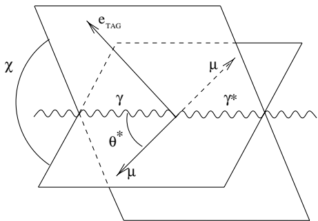
Fig. 2. Illustration of the azimuthal angle \chi for the reaction e^+e^- \rightarrow e^+e^-\gamma^*\gamma^* \rightarrow e^+e^-\mu^+\mu^- in the \gamma^*\gamma^* centre-of-mass system
