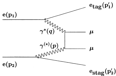
Fig. 1. Diagram of the reaction ee \rightarrow ee\gamma^*\gamma^* \rightarrow ee\mu^+\mu^- . The symbols in brackets denote the four-vectors of the particles
