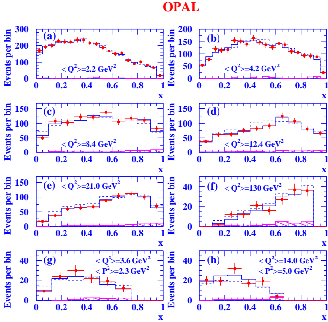
Fig. 6. The measured x distributions for the various samples a SW1, b SW2, c FD1, d FD2, e FD3, f EE, g DB1 and h DB2. The sample definitions are given in Table 1. The points represent the data with the statistical error only. The dashed lines denote the distributions of the Vermaseren Monte Carlo with the background added to it before the unfolding is performed, the full lines are the same distributions after reweighting based on the unfolding procedure, and the hatched histograms represent the background contribution
