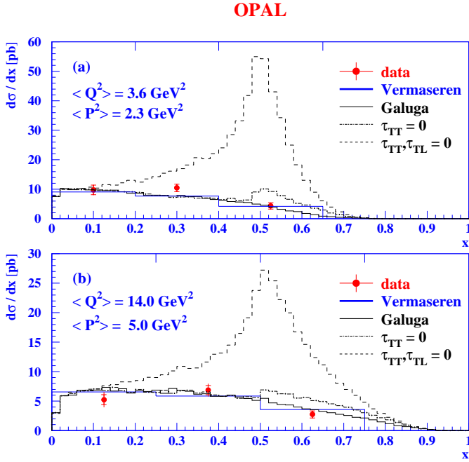
Fig. 11. Differential cross-sections d\sigma/dx unfolded from the data, a for the DB1 sample and b for the DB2 sample. The sample definitions are given in Table 1. The points represent the data with their statistical (inner error bars) and total errors (outer error bars). The full line denotes the differential cross-sections as predicted by the Vermaseren Monte Carlo using the same bins as for the data. The additional three histograms represent the cross-section calculations from the GALUGA Monte Carlo for three different scenarios: the full cross-section (full line), the cross-section obtained for vanishing \tau_{TT} (dot-dash) and the cross-section obtained for vanishing \tau_{TT} and \tau_{TL} (dash), as defined in (2). The tic marks at the top of the figures indicate the bin boundaries
