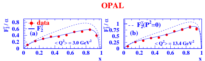
Fig. 10. Structure functions F_2^\gamma normalised by the fine structure constant \alpha for the two combined samples of singly-tagged events. The samples shown are a SW and b FD. The symbols are as defined in Fig. 9
